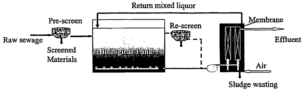
Figure 24 - MemJet MBR Configuration with Gravity Re-screening
